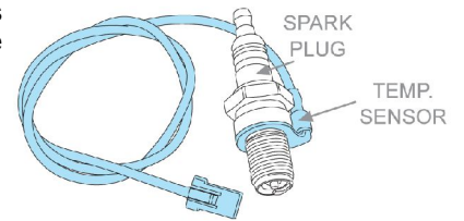
Cylinder Head Temperature Sensor for air-cooled machines
